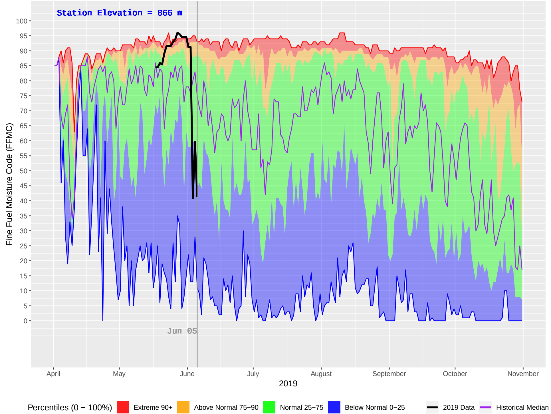
CATFISH (199) : Historical (1986–2018) and Current (2019) Daily Fine Fuel Moisture Code (FFMC)
