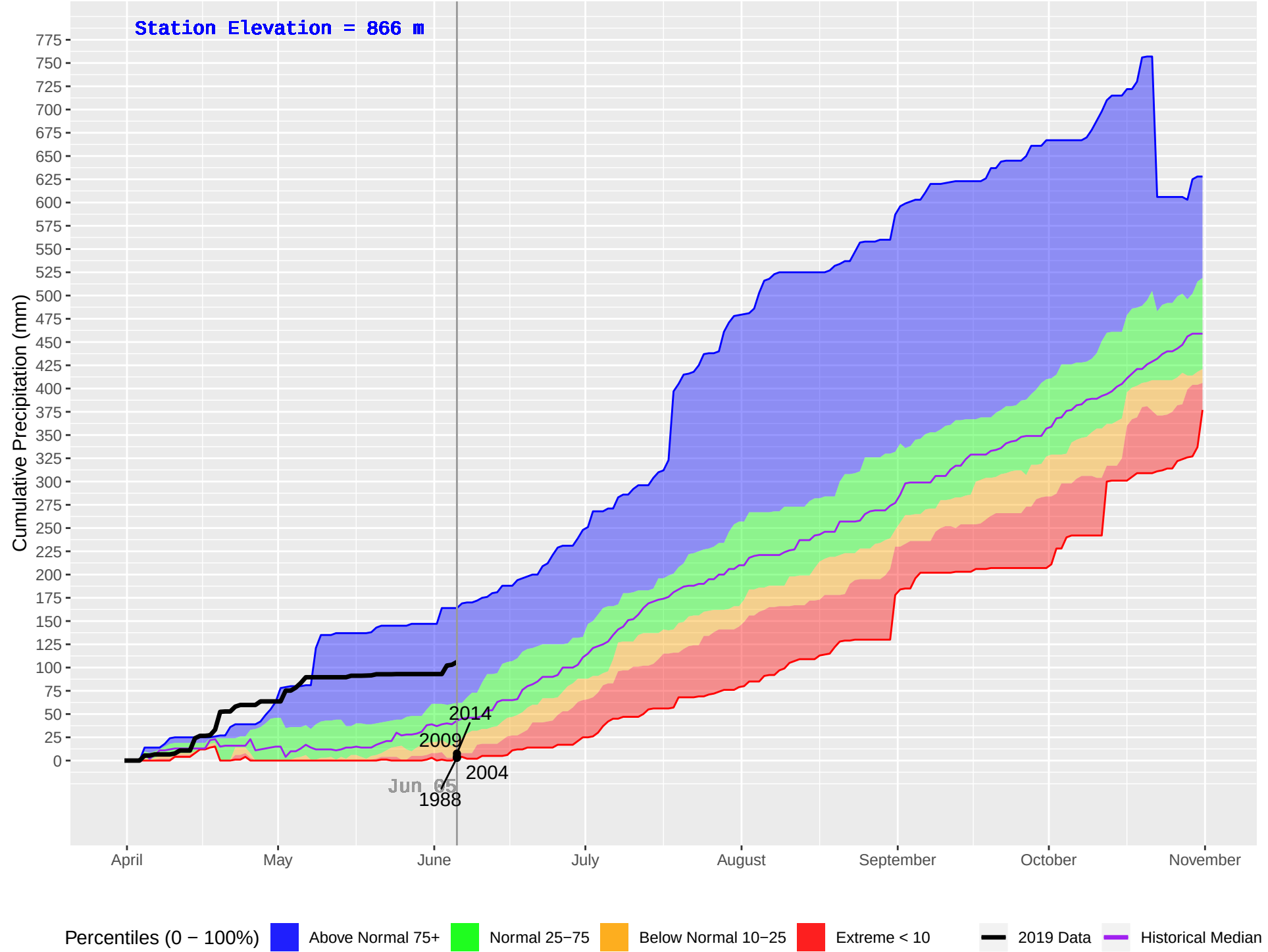
CATFISH (199) : Historical (1986–2018), Current (2019) Daily Cumulative Precipitation
