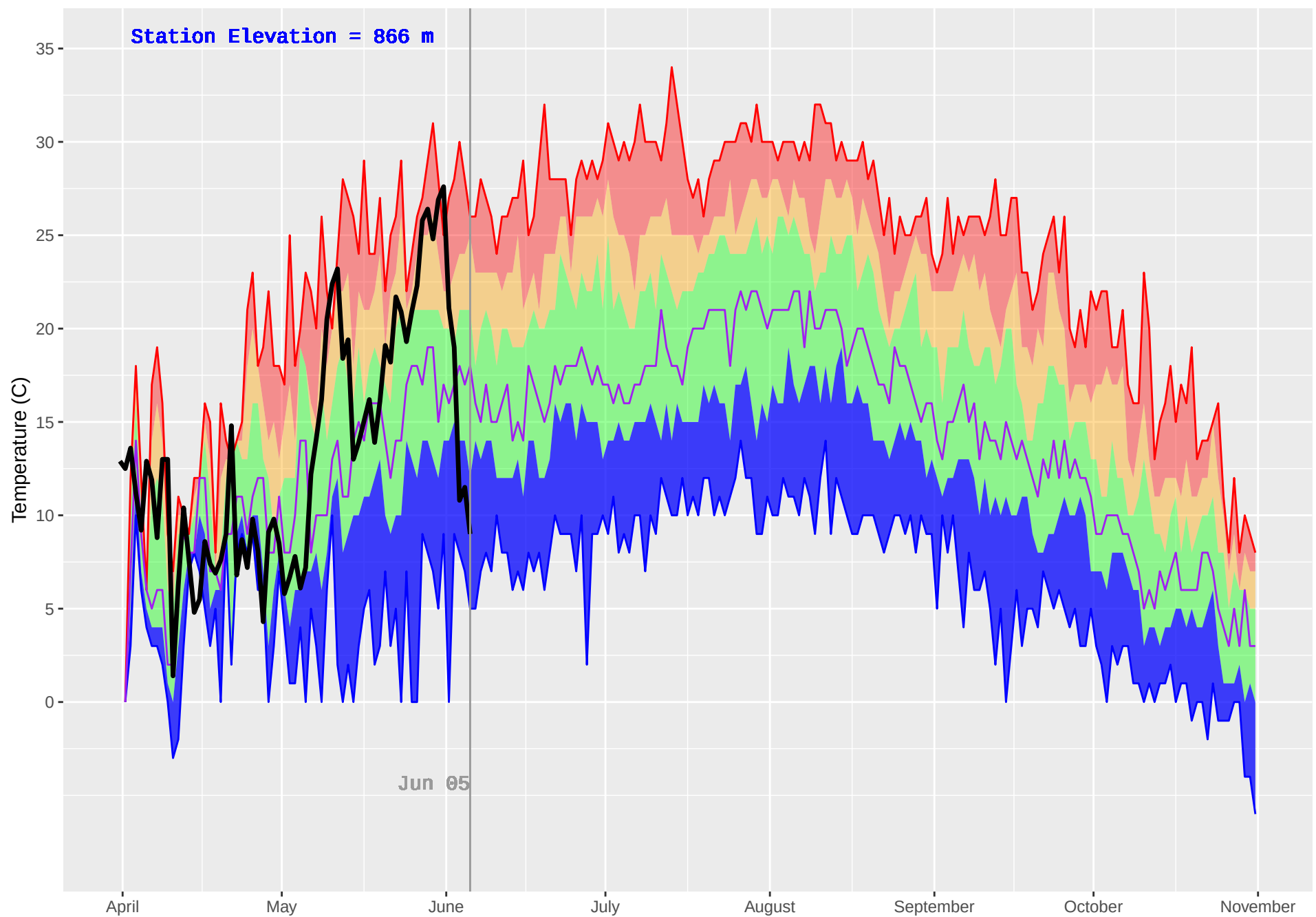
CATFISH (199) : Historical (1986–2018) and Current (2019) Daily Temperature
