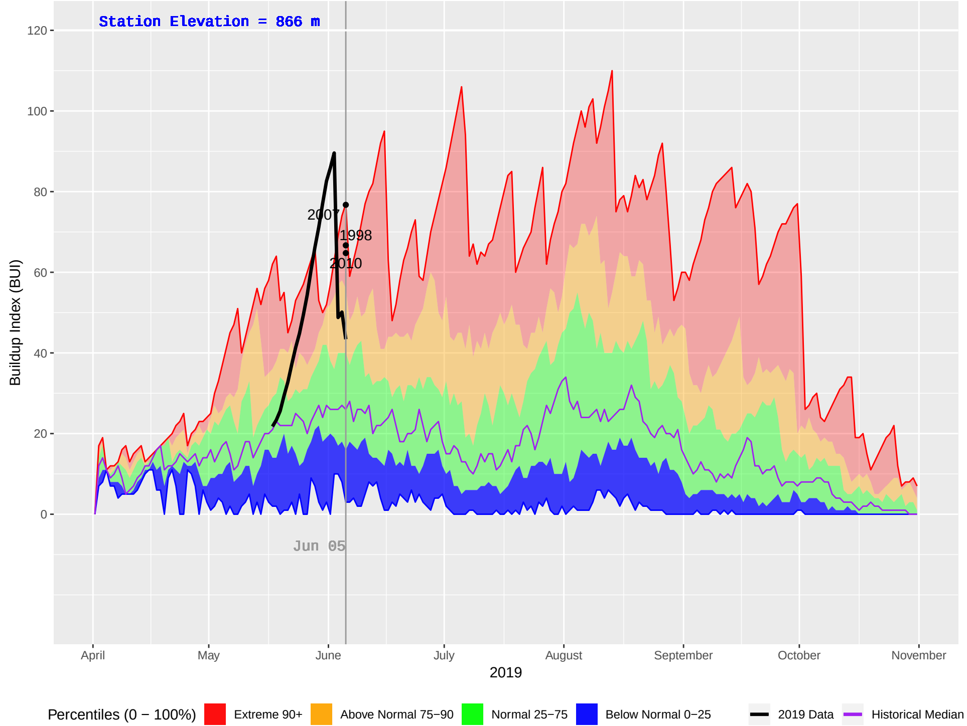
CATFISH (199) : Historical (1986–2018), Current (2019) Daily Buildup Index (BUI)
