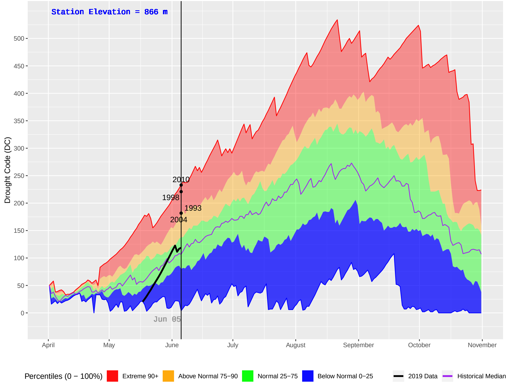
CATFISH (199) : Historical (1986–2018) and Current (2019) Daily Drought Code (DC)
