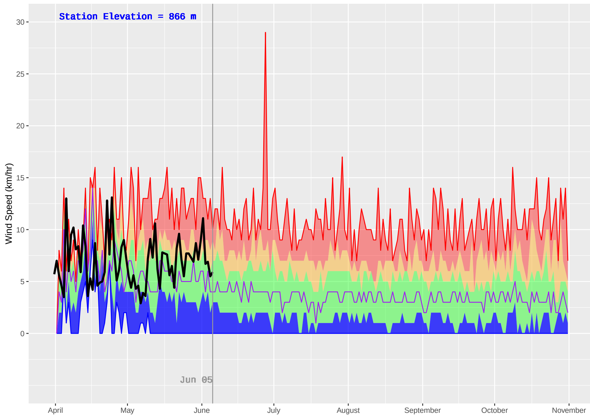
CATFISH (199) : Historical (1986–2018) and Current (2019) Daily Wind Speed
