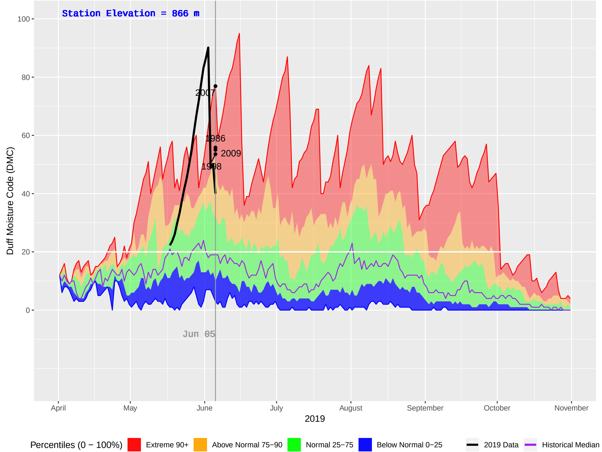
CATFISH (199) : Historical (1986–2018), Current (2019) Daily Duff Moisture Code (DMC)
