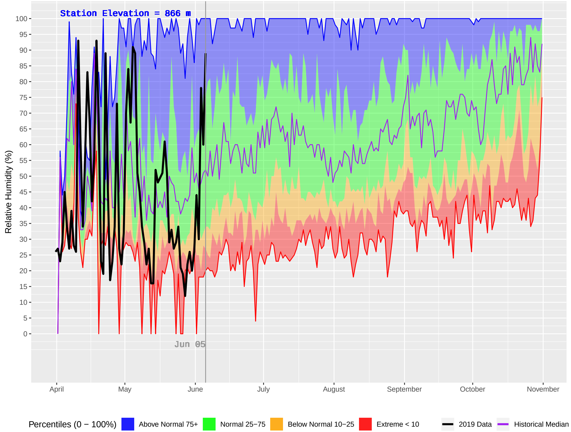
CATFISH (199) : Historical (1986–2018) and Current (2019) Daily Relative Humidity
